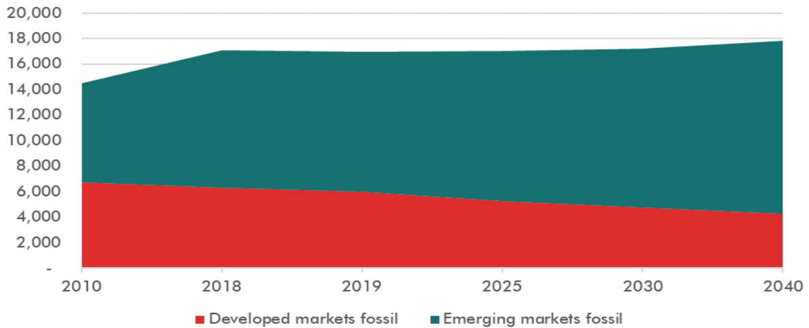
FIGURE 54: FOSSIL FUEL SUPPLY FOR ELECTRICITY GENERATION – STEPS FRAMING TWH
