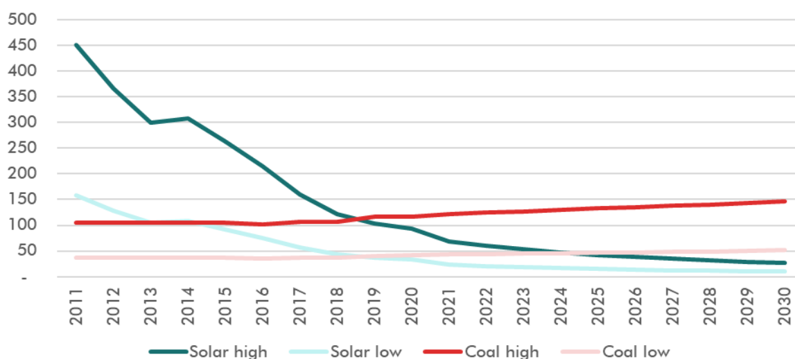
FIGURE 25: SOLAR AND COAL COSTS $ PER MWH
