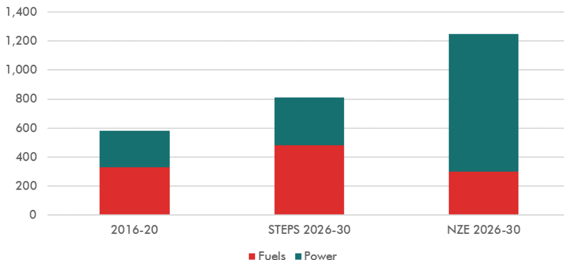
FIGURE 38: ANNUAL ENERGY CAPEX IN THE EMERGING MARKETS EX-CHINA $BN PA
