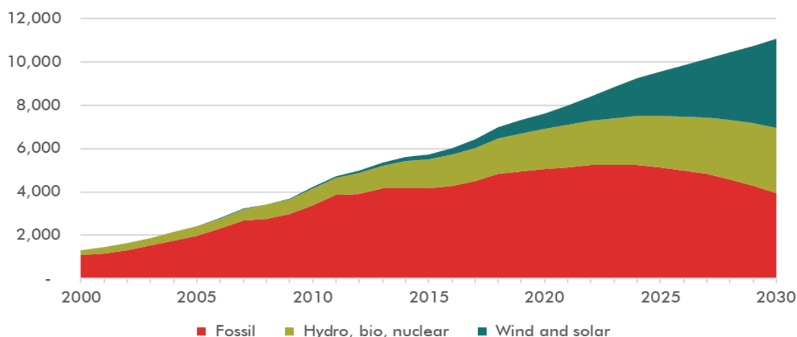
FIGURE 53: CHINA ELECTRICITY SUPPLY ILLUSTRATION TWH
